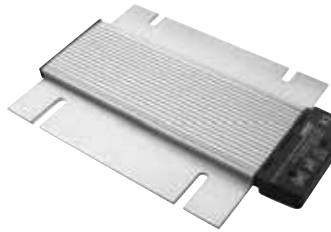
Electric Heater 230V, 380Watts Size 198×297mm
